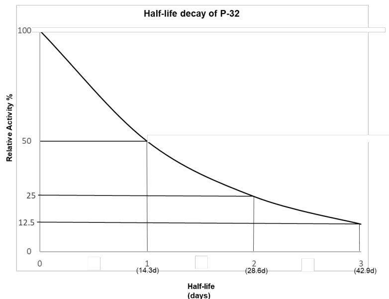
Fig. 5. Decay of Phosphorus-32
