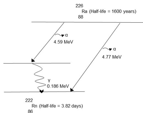
Figure 2. Decay Scheme for Radium -226
