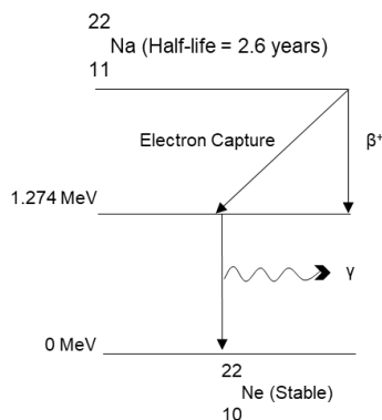
Fig. 4. Decay Scheme for Sodium-22
