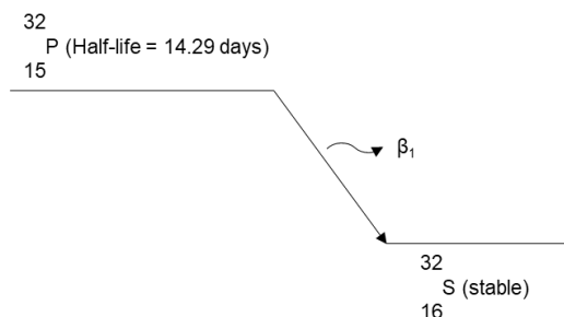
Fig 3. Decay Scheme for Phosphorus-32
