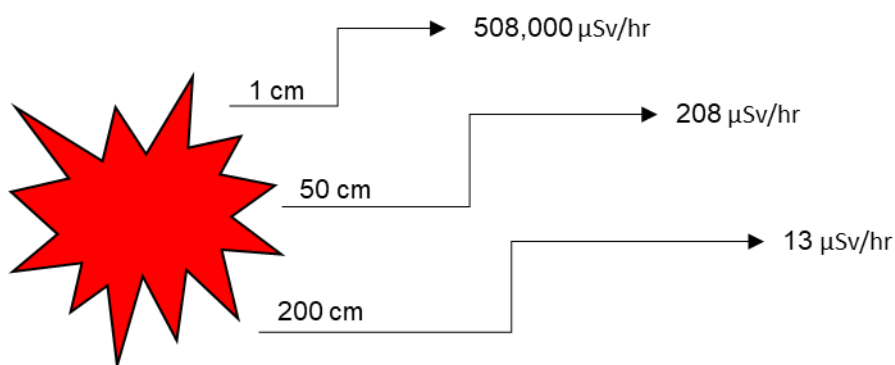
Fig. 6. Effect of Distance on Radiation Intensity (μSv/hr)
